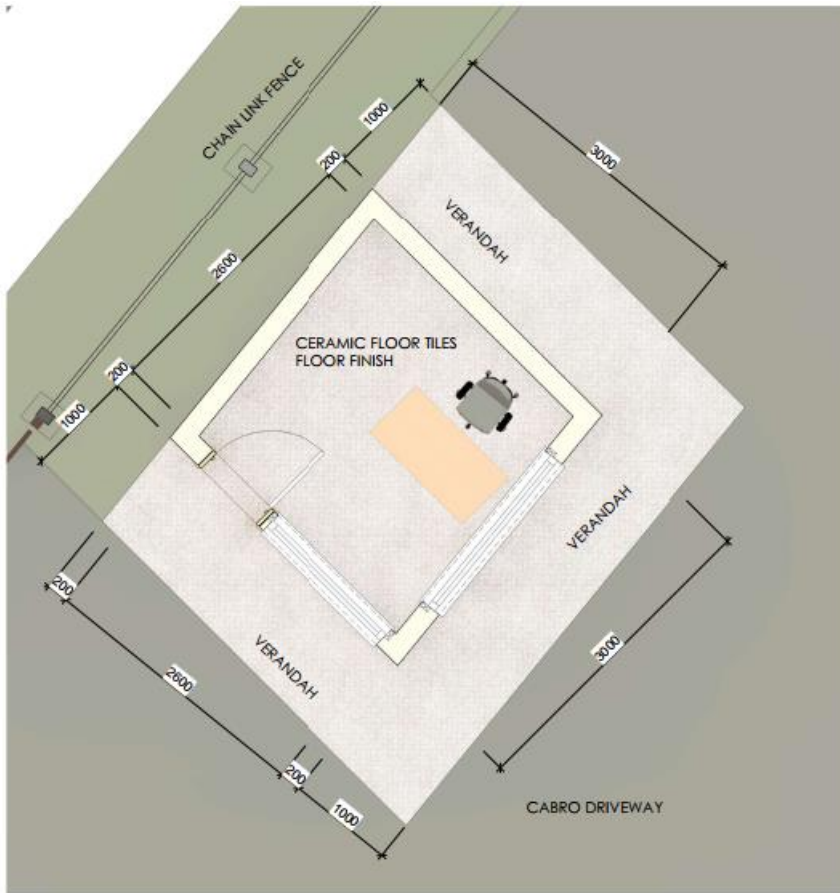
GUARD HOUSE GROUND FLOOR LAYOUT 1:20
